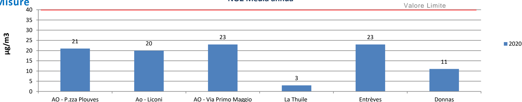
NO 2 Media annua
