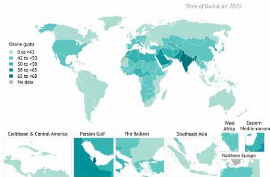
FIGURE 5 Global map of population-weighted average seasonal 8-hour daily maximum ozone concentrations in 2019.
