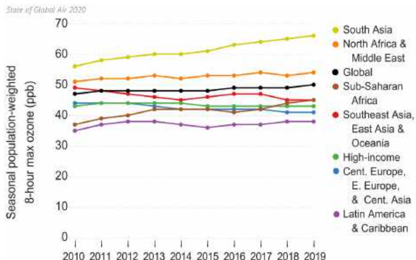
FIGURE 6 Trends in population-weighted average seasonal 8-hour maximum ozone concentration globally and in the GBD Super Regions, 2010–2019.
