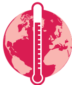
Figure 4: Different threat types in the Living Planet Database
