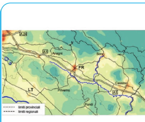
\text{PM}_{25} : media annua 2018 dominio Valle del Sacco (1 km x 1 km)
