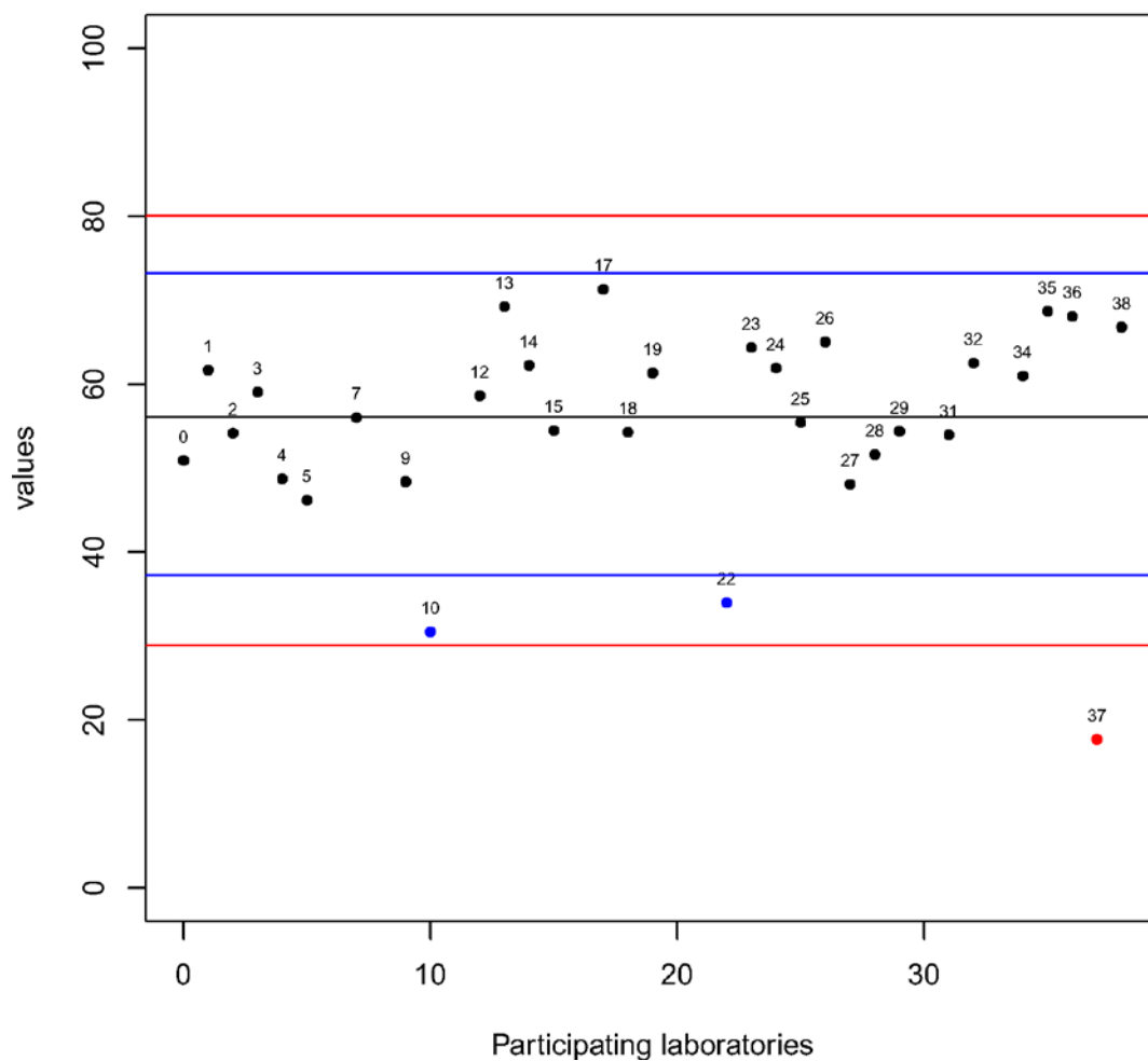
Figure 3.22 Results of Exercise 1 (%). Black line is equal to \text{median}_i x_i , blue lines are equal to \pm 2 * z\text{-score} and red lines are equal to \pm 3 * z\text{-score} . Black dots represent results classified 'S', blue dots those classified 'Q' and red dots the results classified 'U'.
