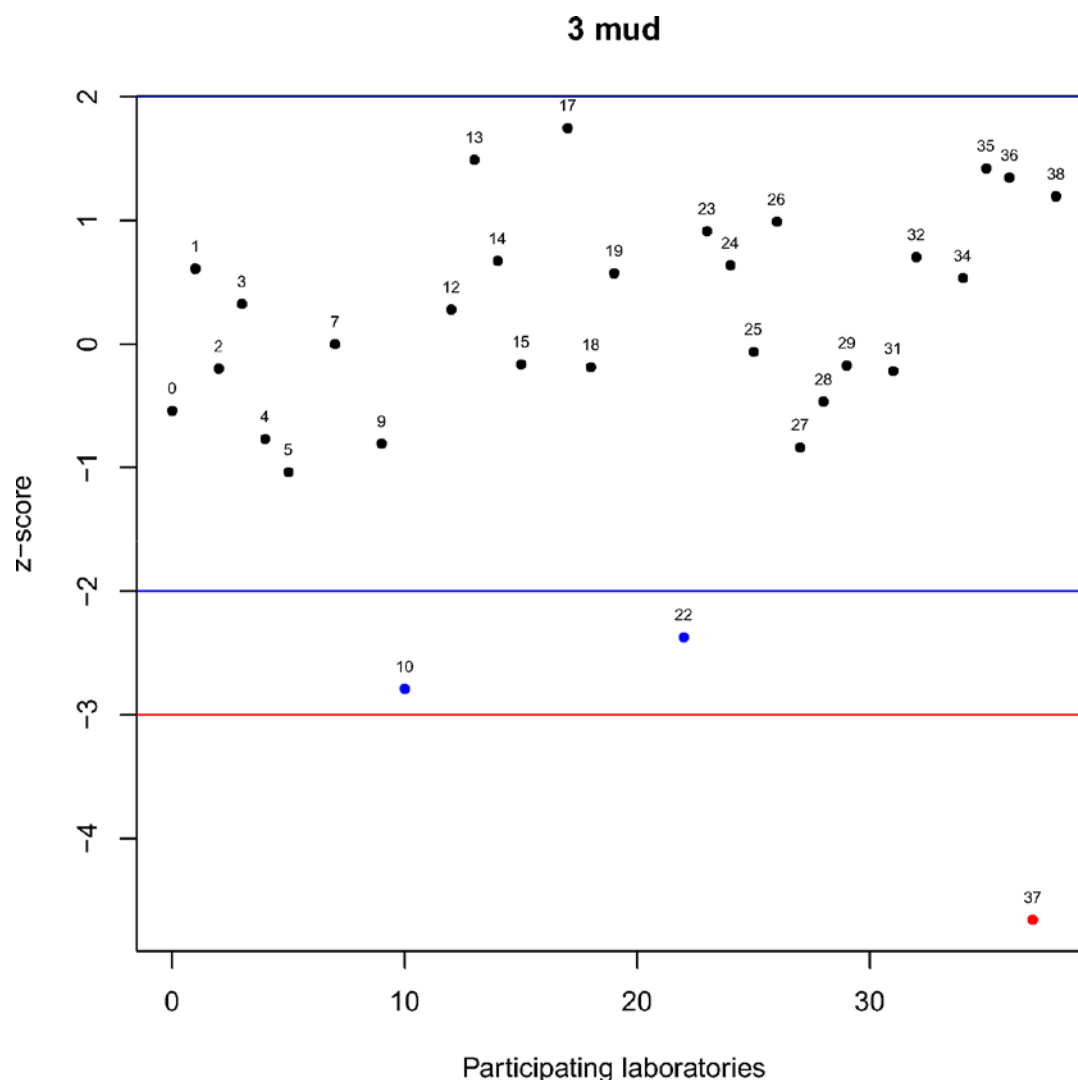
Figure 3.21 Results of Exercise 1 (z-score). Blue lines are equal to \pm 2 * z\text{-score} and red lines are equal to \pm 3 * z\text{-score} . Black dots represent results classified 'S', blue dots those classified 'Q' and red dots the results classified 'U'.
