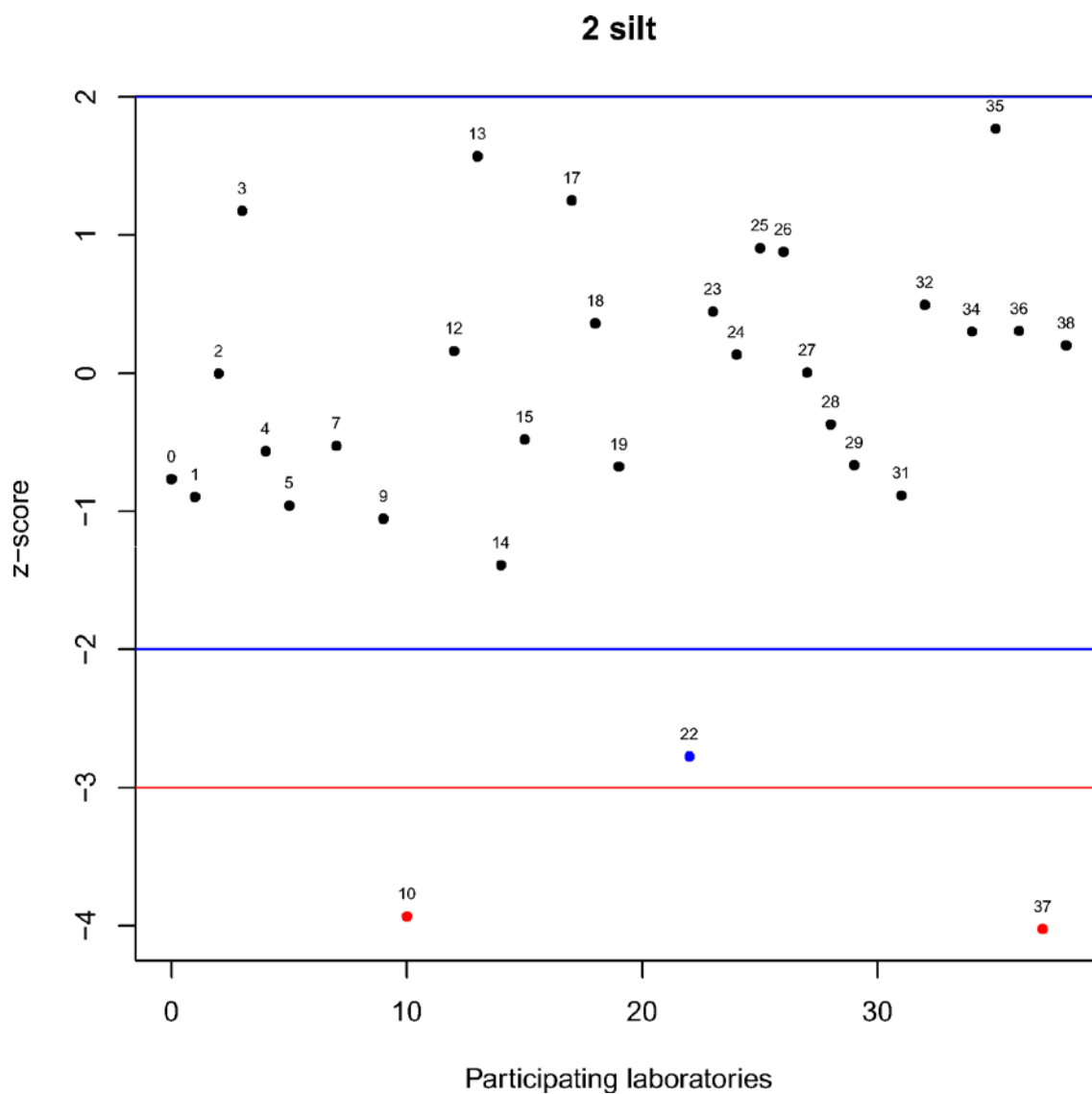
Figure 3.15 Results of Exercise 1 (z-score). Blue lines are equal to \pm 2 \cdot z\text{-score} and red lines are equal to \pm 3 \cdot z\text{-score} . Black dots represent results classified 'S', blue dots those classified 'Q' and red dots the results classified 'U'.
