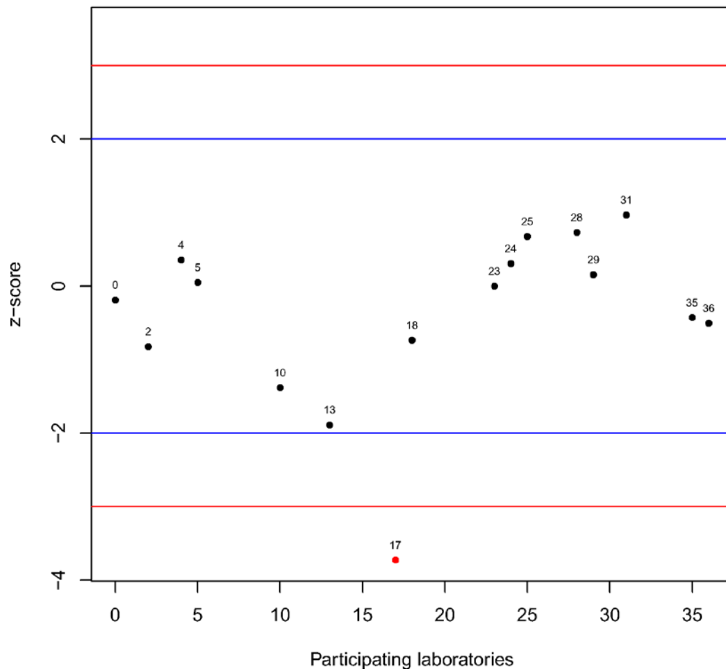
Figure 3.29 Fraction >63 \mu\text{m} (z-score). Blue lines are equal to \pm 2 * \text{z-score} and red lines are equal to \pm 3 * \text{z-score} . Numbers represent assigned lab number, black dots represent results classified 'S', blue dots those classified 'Q' and red dots the results classified 'U'.
