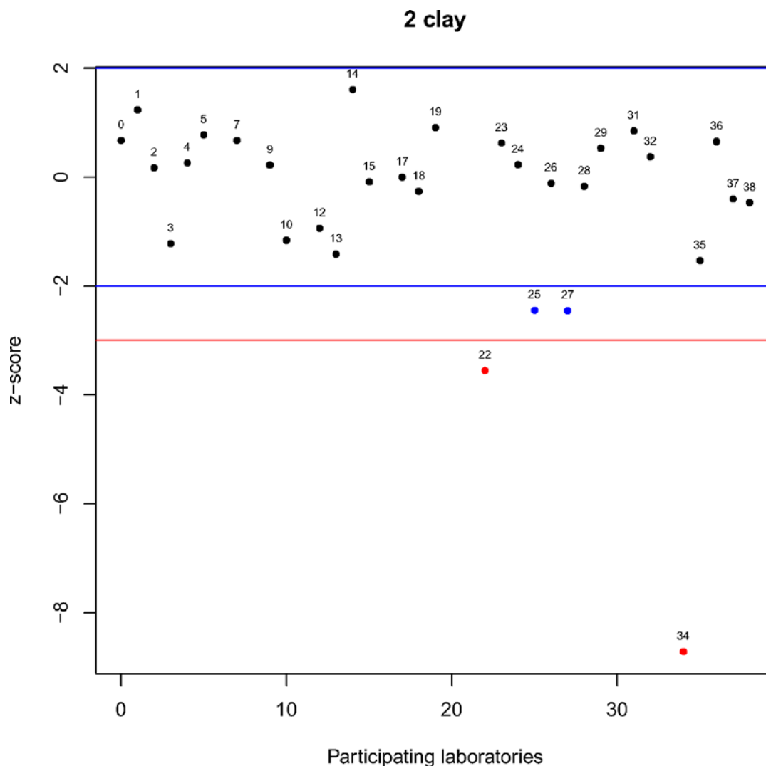
Figure 3.17 Results of Exercise 1 (z-score). Blue lines are equal to \pm 2 * z-score and red lines are equal to \pm 3 * z-score. Black dots represent results classified 'S', blue dots those classified 'Q' and red dots the results classified 'U'.
