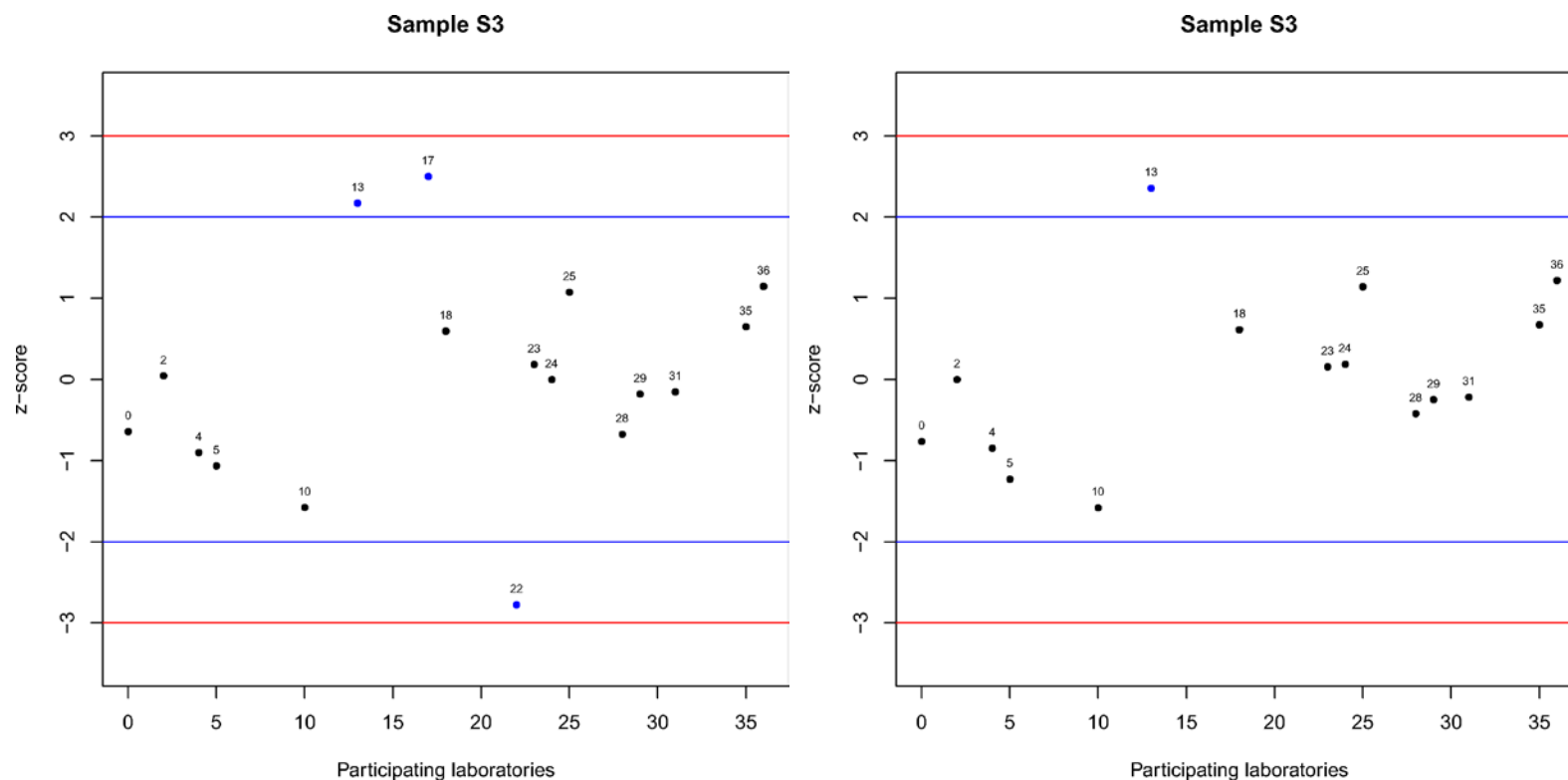
Figure 3.37 Fraction < 63 \mu\text{m} without and with ultrasonic treatment (z-score). Blue lines are equal to \pm 2 * z\text{-score} and red lines are equal to \pm 3 * z\text{-score} . Numbers represent assigned lab number, black dots represent results classified 'S', blue dots those classified 'Q' and red dots the results classified 'U'.
