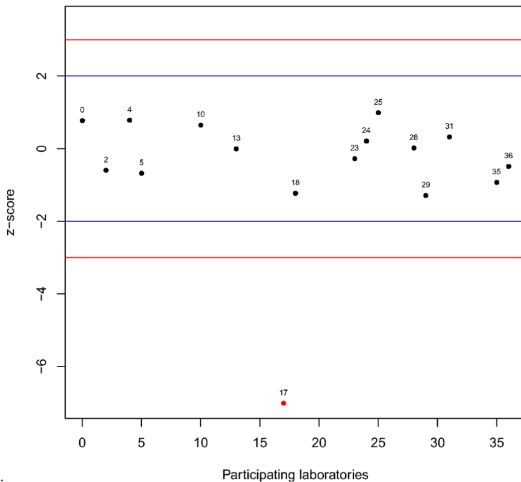
Figure 3.27 Fraction >63 \mu\text{m} (z-score). Blue lines are equal to \pm 2 * \text{z-score} and red lines are equal to \pm 3 * \text{z-score} . Numbers represent assigned lab number, black dots represent results classified 'S', blue dots those classified 'Q' and red dots the results classified 'U'.
