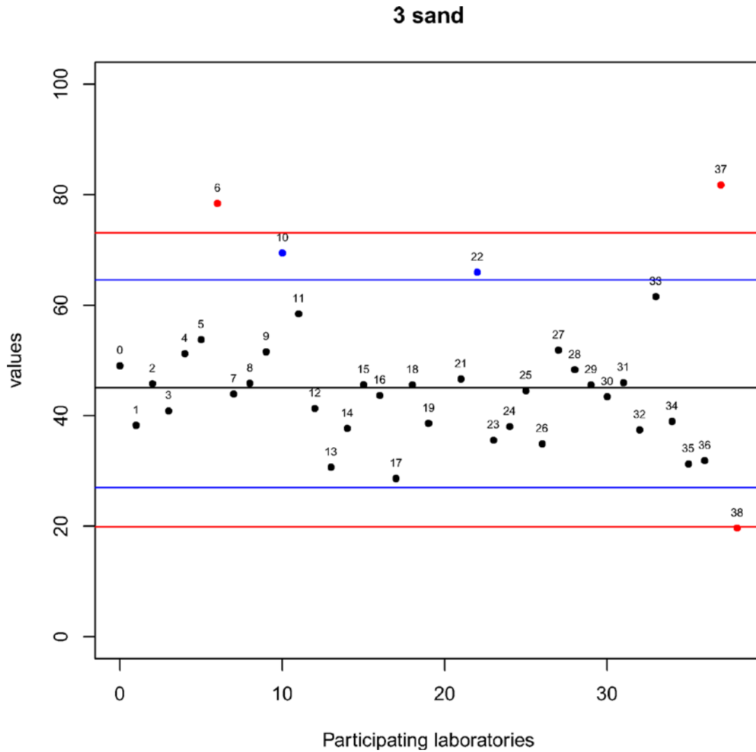
Figure 3.20 Results of Exercise 1 (%). Black line is equal to median x_i , blue lines are equal to \pm 2 * z-score and red lines are equal to \pm 3 * z-score. Black dots represent results classified 'S', blue dots those classified 'Q' and red dots the results classified 'U'.
