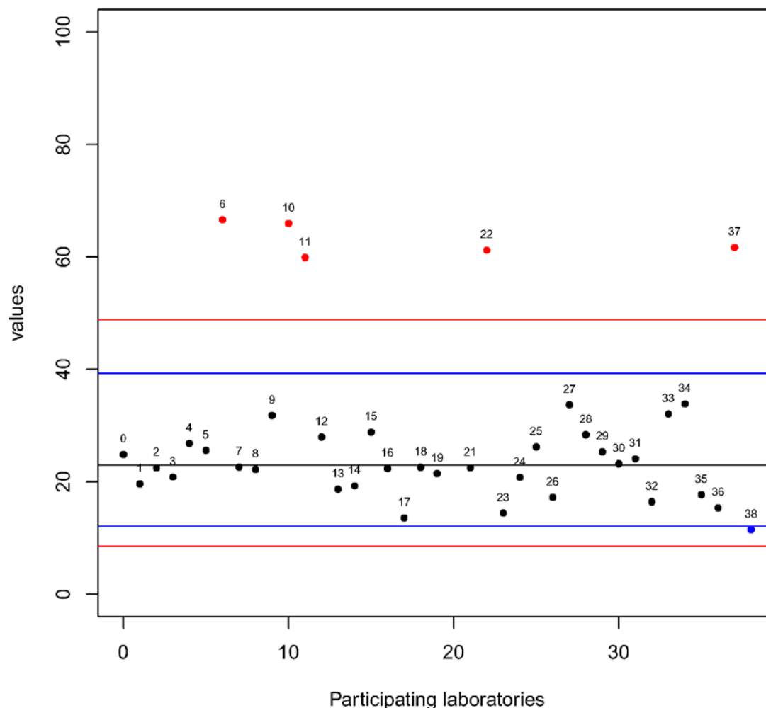
Figure 3.12 Results of Exercise 1 (%). Black line is equal to median x_i , blue lines are equal to \pm 2 * z -score and red lines are equal to \pm 3 * z -score. Black dots represent results classified 'S', blue dots those classified 'Q' and red dots the results classified 'U'.
