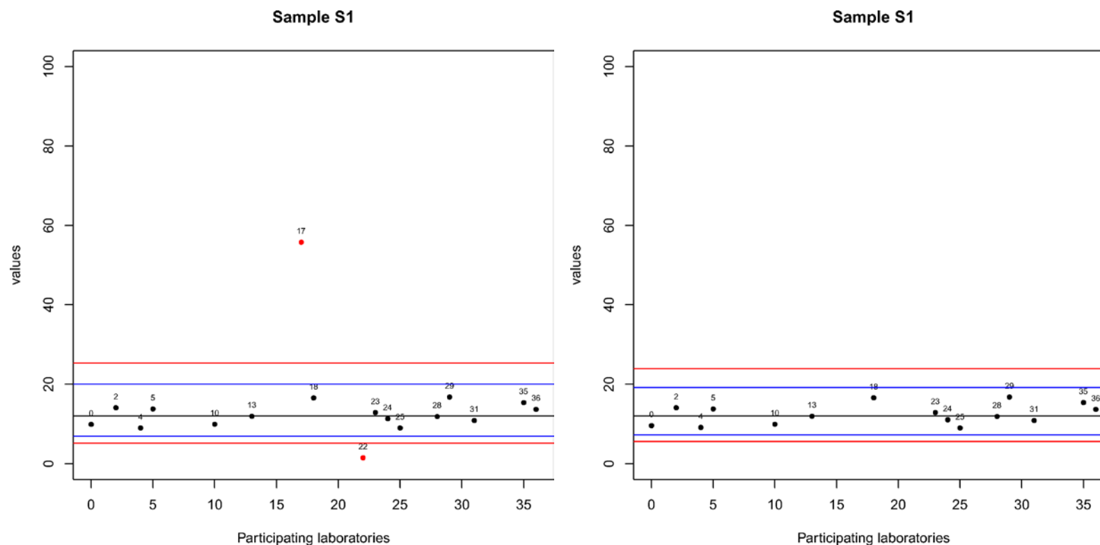
Figure 3.34 Fraction <63 \mu\text{m} without and with ultrasonic treatment (%). Black line is equal to median , blue lines are equal to \pm 2 * z-score and red lines are equal to \pm 3 * z-score . Numbers represent assigned lab number, black dots represent results classified 'S', blue dots those classified 'Q' and red dots the results classified 'U'.
