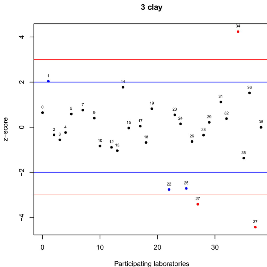
Figure 3.25 Results of Exercise 1 (z-score). Blue lines are equal to \pm 2 * z-score and red lines are equal to \pm 3 * z-score. Black dots represent results classified 'S', blue dots those classified 'Q' and red dots the results classified 'U'.
