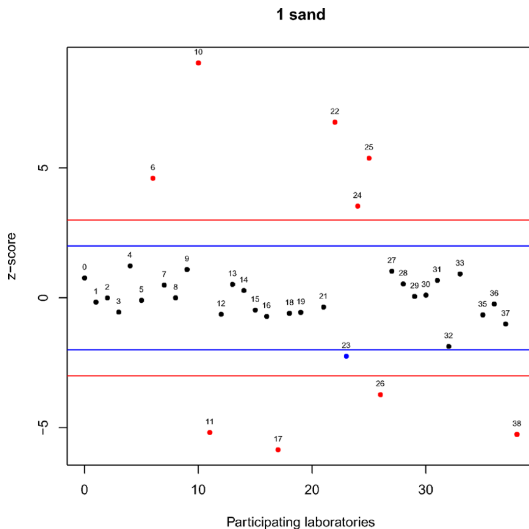
Figure 3.3 Results of Exercise 1 (z-score). Blue lines are equal to \pm 2 \cdot z\text{-score} and red lines are equal to \pm 3 \cdot z\text{-score} . Black dots represent results classified 'S', blue dots those classified 'Q' and red dots the results classified 'U'.
