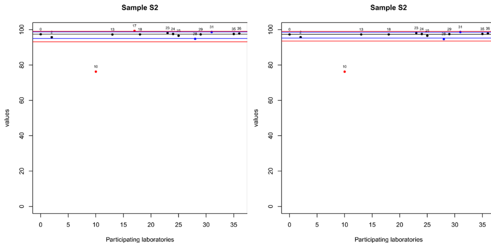
Figure 3.48 Fraction <250 µm without and with ultrasonic treatment (%). Black line is equal to median i x i , blue lines are equal to ± 2 * z-score and red lines are equal to ± 3 * z-score . Numbers represent assigned lab number, black dots represent results classified 'S', blue dots those classified 'Q' and red dots the results classified 'U'.
