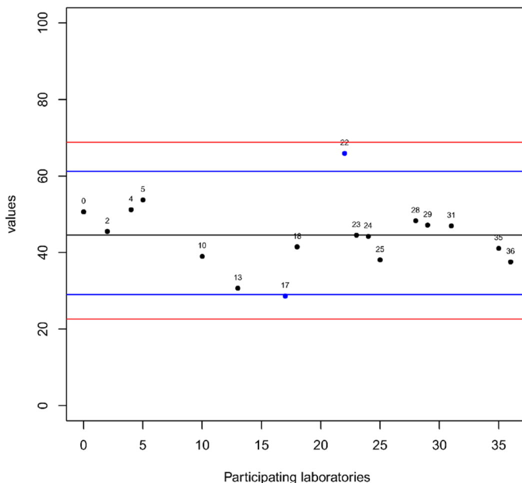
Figure 3.32 Fraction >63 \mu\text{m} (%). Black line is equal to median i x_p , blue lines are equal to \pm 2 * z\text{-score} and red lines are equal to \pm 3 * z\text{-score} . Numbers represent assigned lab number, black dots represent results classified 'S', blue dots those classified 'Q' and red dots the results classified 'U'.
