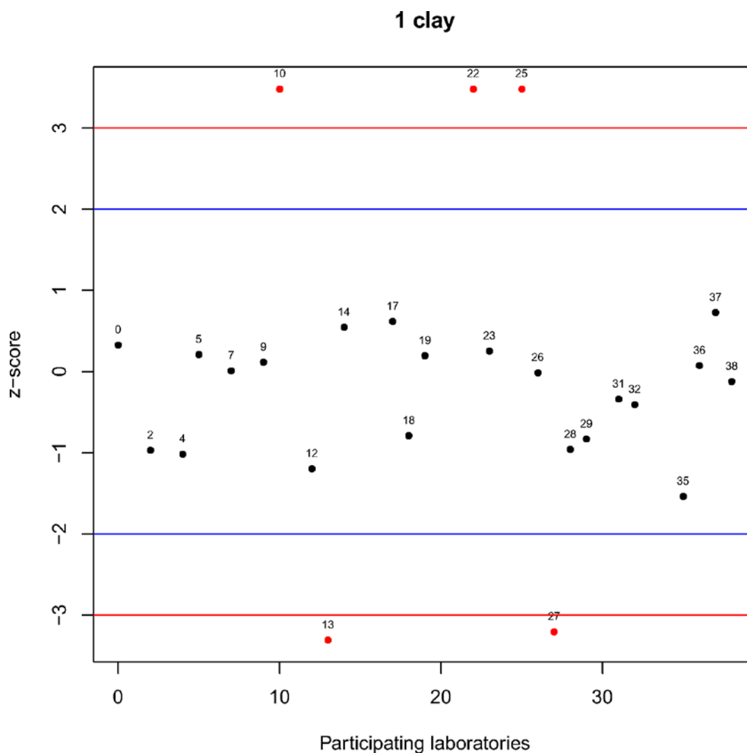
Figure 3.9 Results of Exercise 1 (z-score). Blue lines are equal to \pm 2 * z-score and red lines are equal to \pm 3 * z-score. Black dots represent results classified 'S', blue dots those classified 'Q' and red dots the results classified 'U'.
