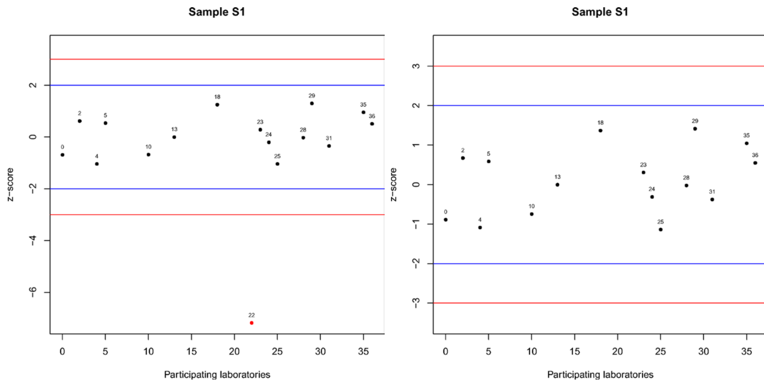
Figure 3.33 Fraction < 63 \mu\text{m} without and with ultrasonic treatment (z-score). Blue lines are equal to \pm 2 * z\text{-score} and red lines are equal to \pm 3 * z\text{-score} . Numbers represent assigned lab number, black dots represent results classified 'S', blue dots those classified 'Q' and red dots the results classified 'U'.
