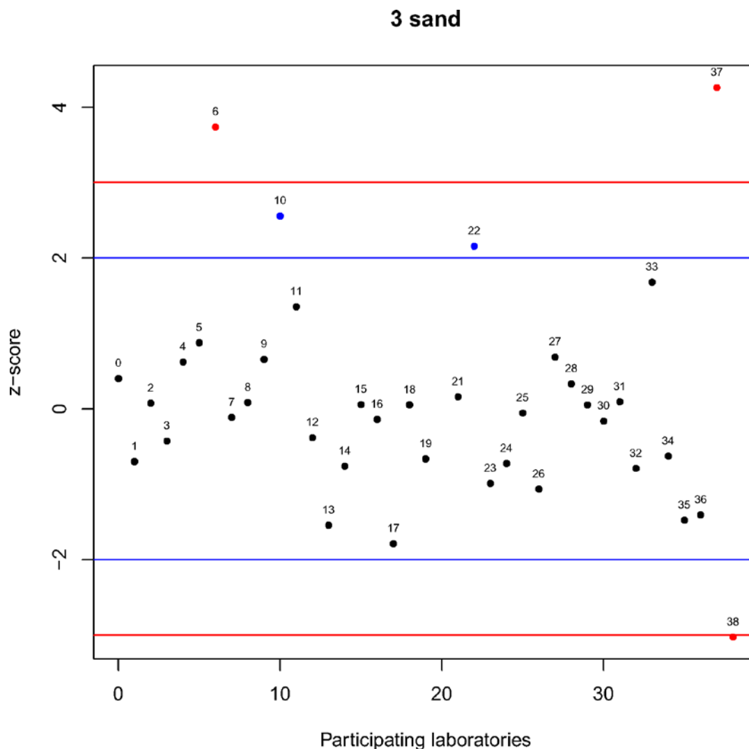
Figure 3.19 Results of Exercise 1 (z-score). Blue lines are equal to \pm 2 * z\text{-score} and red lines are equal to \pm 3 * z\text{-score} . Black dots represent results classified 'S', blue dots those classified 'Q' and red dots the results classified 'U'.
