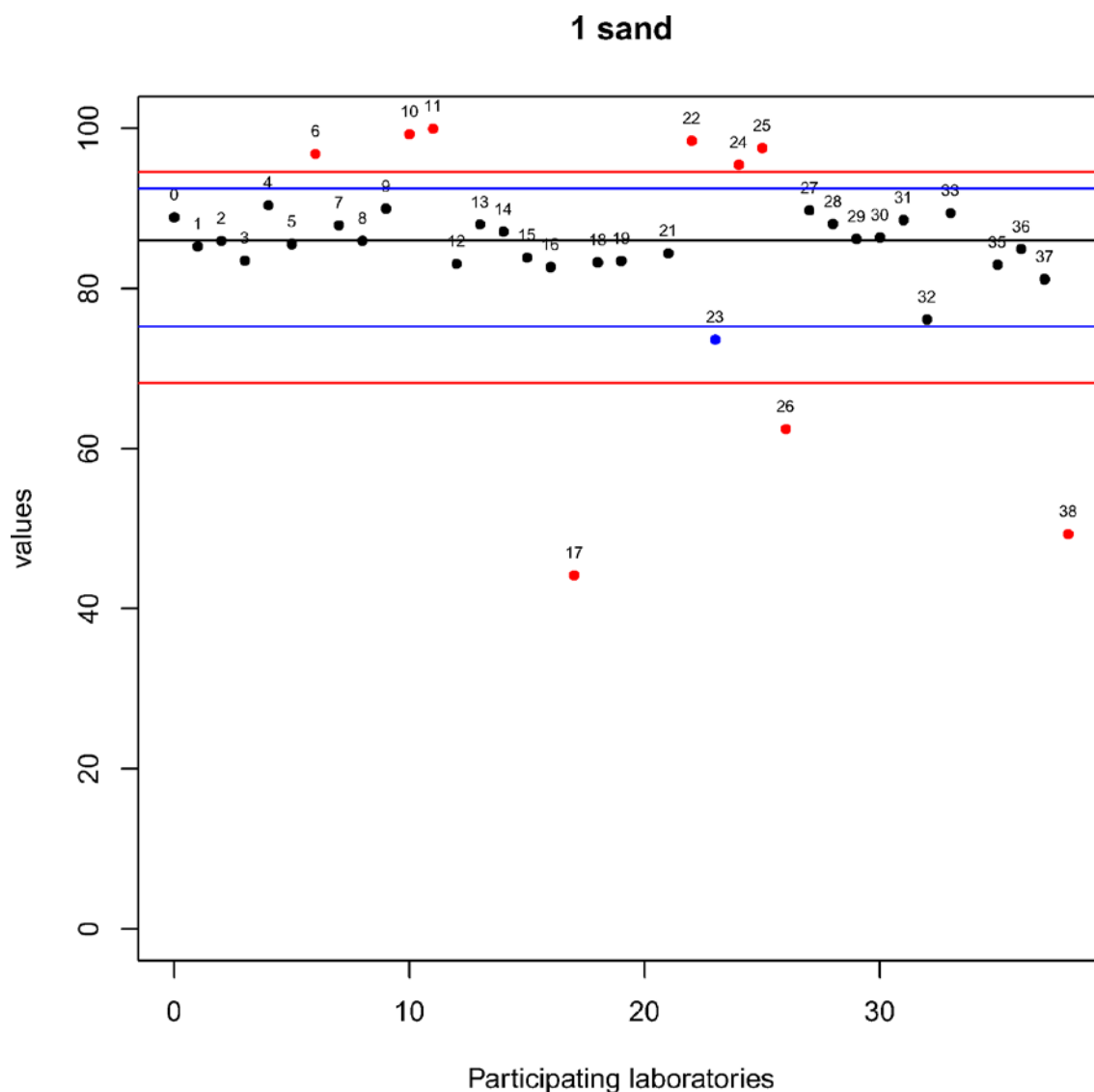
Figure 3.4 Results of Exercise 1 (%). Black line is equal to median, x_i , blue lines are equal to \pm 2 * z -score and red lines are equal to \pm 3 * z -score. Black dots represent results classified 'S', blue dots those classified 'Q' and red dots the results classified 'U'.
