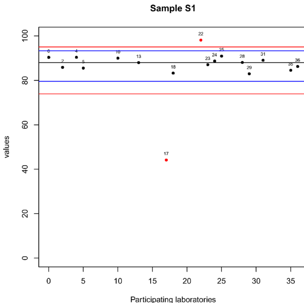
Figure 3.28 Fraction >63 \mu\text{m} (%). Black line is equal to median i x_i , blue lines are equal to \pm 2 * z\text{-score} and red lines are equal to \pm 3 * z\text{-score} . Numbers represent assigned lab number, black dots represent results classified 'S', blue dots those classified 'Q' and red dots the results classified 'U'.
