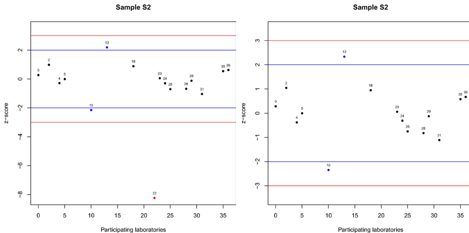
Figure 3.35 Fraction < 63 \mu\text{m} without and with ultrasonic treatment (z-score). Blue lines are equal to \pm 2 * z\text{-score} and red lines are equal to \pm 3 * z\text{-score} . Numbers represent assigned lab number, black dots represent results classified 'S', blue dots those classified 'Q' and red dots the results classified 'U'.
