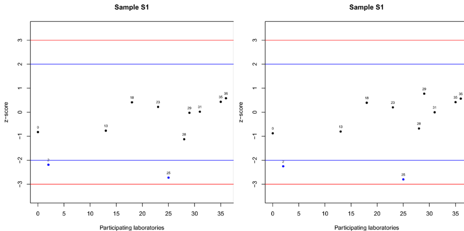
Figure 3.45 Fraction < 250 \mu\text{m} without and with ultrasonic treatment (z-score). Blue lines are equal to \pm 2 * \text{z-score} and red lines are equal to \pm 3 * \text{z-score} . Numbers represent assigned lab number, black dots represent results classified 'S', blue dots those classified 'Q' and red dots the results classified 'U'.
