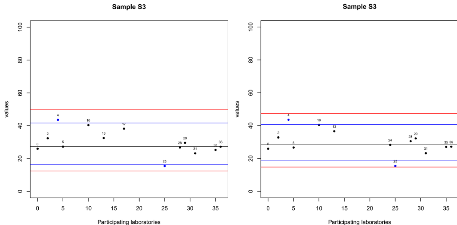
Figure 3.44 Fraction <22.5 μm without and with ultrasonic treatment (%). Black line is equal to median x_i , blue lines are equal to \pm 2 * z -score and red lines are equal to \pm 3 * z -score. Numbers represent assigned lab number, black dots represent results classified 'S', blue dots those classified 'Q' and red dots the results classified 'U'.
