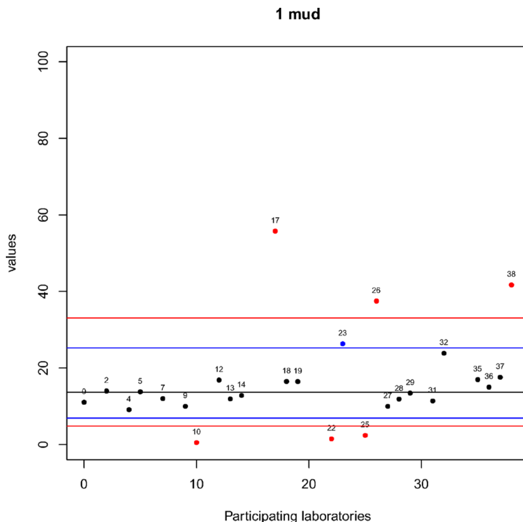
Figure 3.6 Results of Exercise 1 (%). Black line is equal to median x_i , blue lines are equal to \pm 2 * z\text{-score} and red lines are equal to \pm 3 * z\text{-score} . Black dots represent results classified 'S', blue dots those classified 'Q' and red dots the results classified 'U'.
