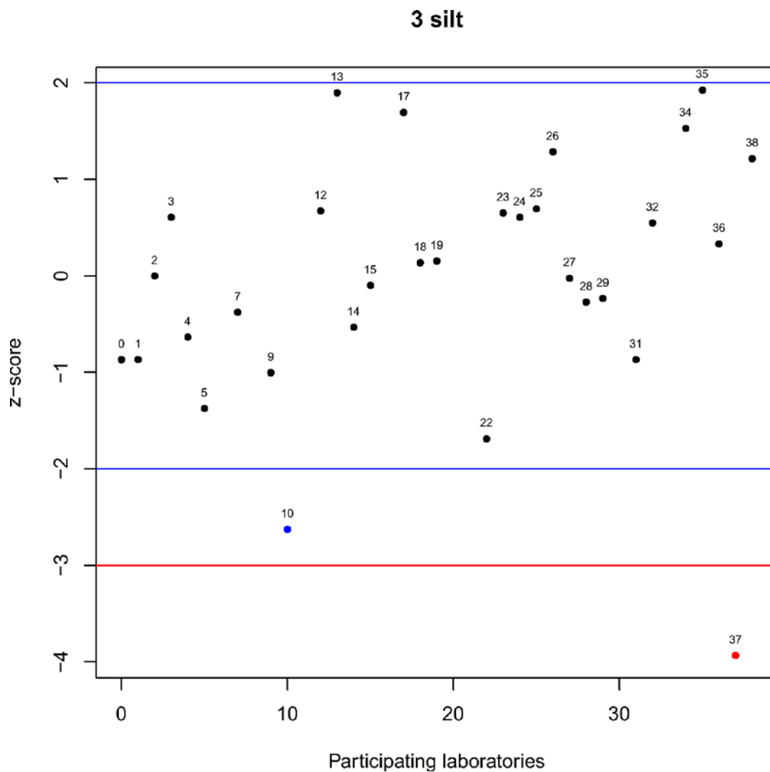
Figure 3.23 Results of Exercise 1 (z-score). Blue lines are equal to \pm 2 * z\text{-score} and red lines are equal to \pm 3 * z\text{-score} . Black dots represent results classified 'S', blue dots those classified 'Q' and red dots the results classified 'U'.
