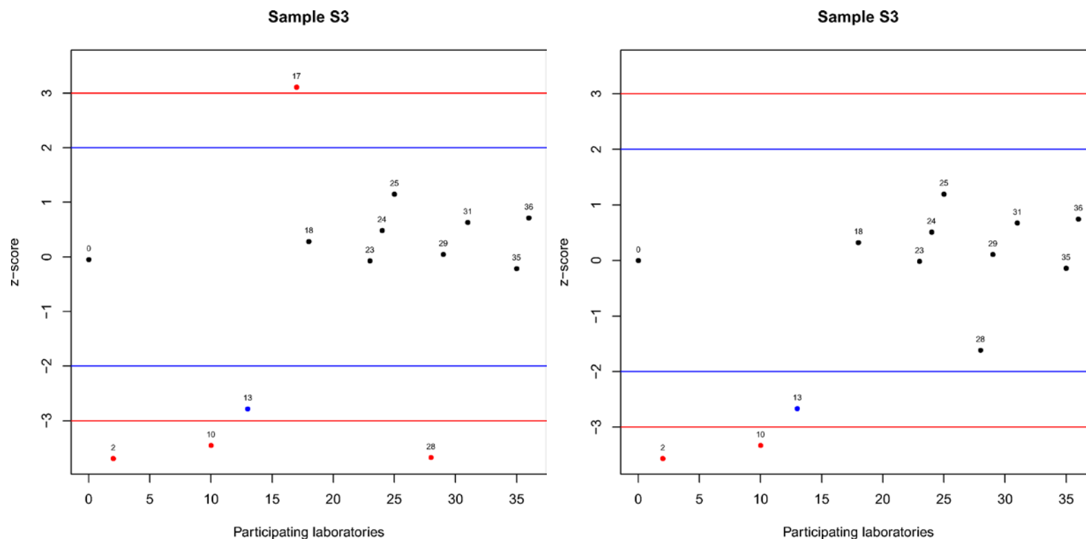
Figure 3.49 Fraction < 250 \mu\text{m} without and with ultrasonic treatment (z-score). Blue lines are equal to \pm 2 * \text{z-score} and red lines are equal to \pm 3 * \text{z-score} . Numbers represent assigned lab number, black dots represent results classified 'S', blue dots those classified 'Q' and red dots the results classified 'U'.
