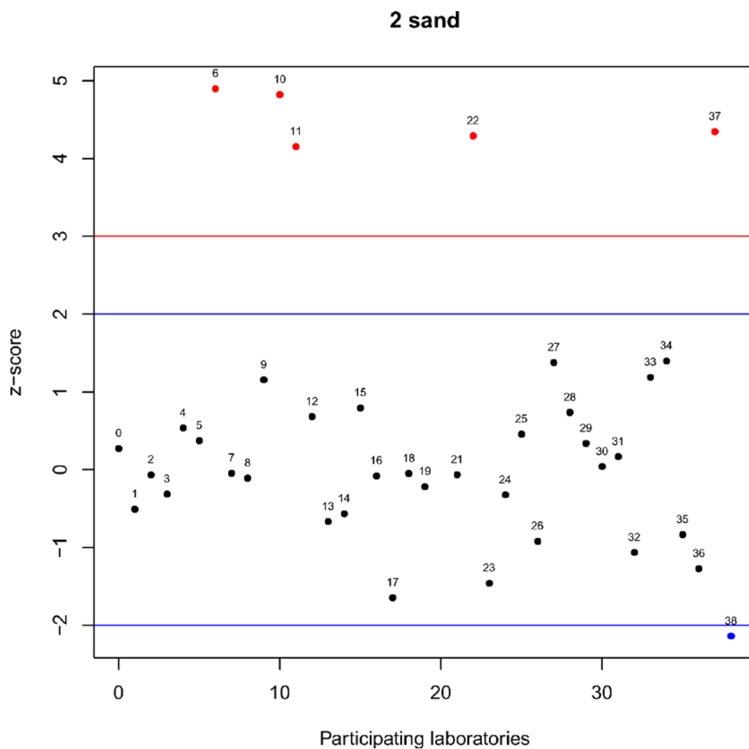
Figure 3.11 Results of Exercise 1 (z-score). Blue lines are equal to \pm 2 * z\text{-score} and red lines are equal to \pm 3 * z\text{-score} . Black dots represent results classified 'S', blue dots those classified 'Q' and red dots the results classified 'U'.
