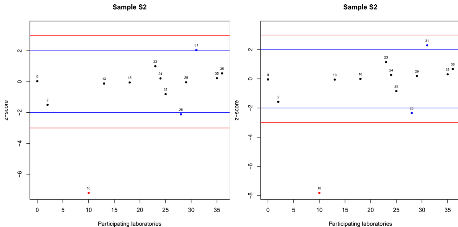
Figure 3.47 Fraction < 250 \mu\text{m} without and with ultrasonic treatment (z-score). Blue lines are equal to \pm 2 * \text{z-score} and red lines are equal to \pm 3 * \text{z-score} . Numbers represent assigned lab number, black dots represent results classified 'S', blue dots those classified 'Q' and red dots the results classified 'U'.
