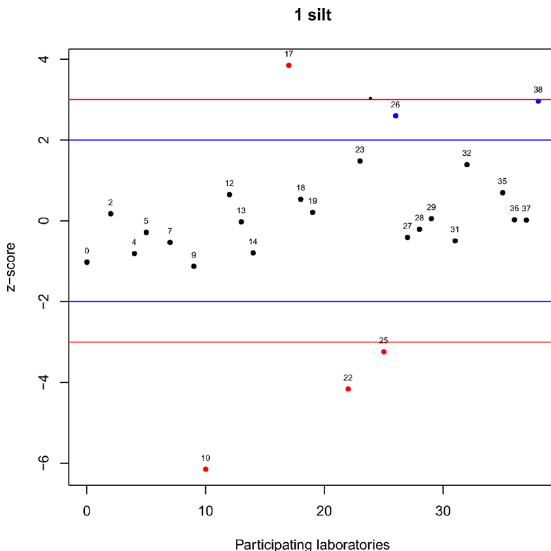
Figure 3.7 Results of Exercise 1 (z-score). Blue lines are equal to \pm 2 \cdot z\text{-score} and red lines are equal to \pm 3 \cdot z\text{-score} . Black dots represent results classified 'S', blue dots those classified 'Q' and red dots the results classified 'U'.
