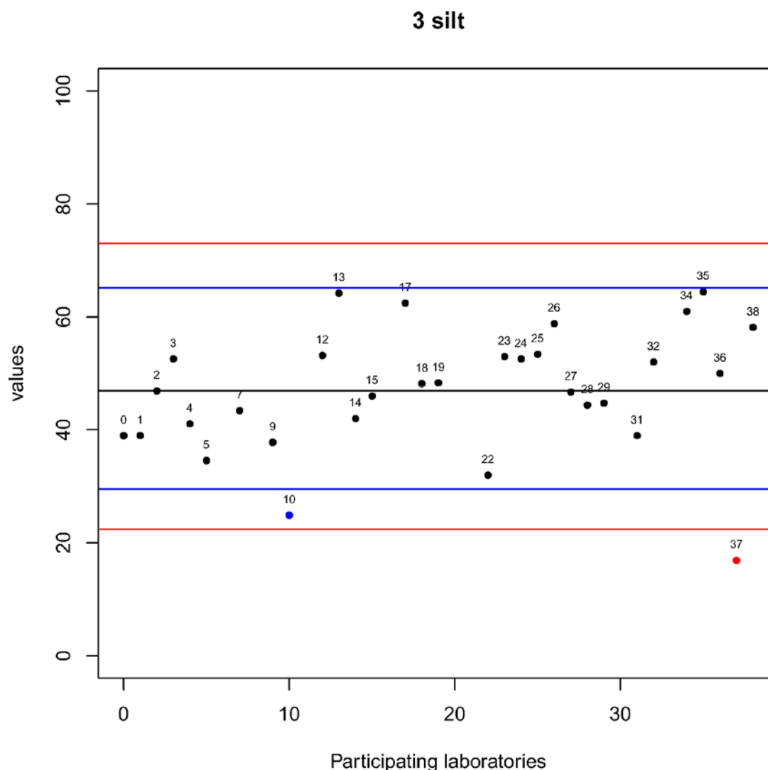
Figure 3.24 Results of Exercise 1 (%). Black line is equal to \text{median}_i x_i , blue lines are equal to \pm 2 * z\text{-score} and red lines are equal to \pm 3 * z\text{-score} . Black dots represent results classified 'S', blue dots those classified 'Q' and red dots the results classified 'U'.
