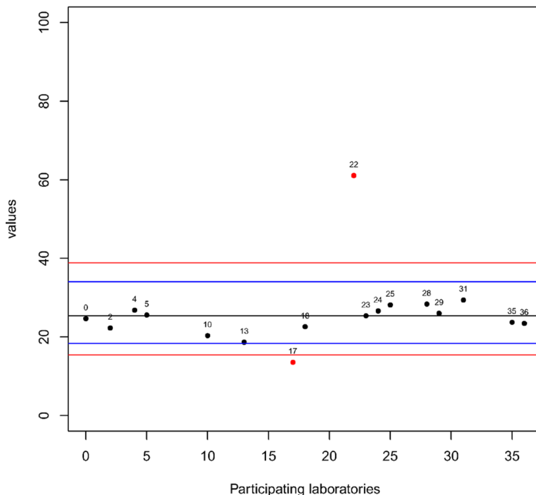
Figure 3.30 Fraction >63 \mu\text{m} (%). Black line is equal to median i x_i , blue lines are equal to \pm 2 * z\text{-score} and red lines are equal to \pm 3 * z\text{-score} . Numbers represent assigned lab number, black dots represent results classified 'S', blue dots those classified 'Q' and red dots the results classified 'U'.
