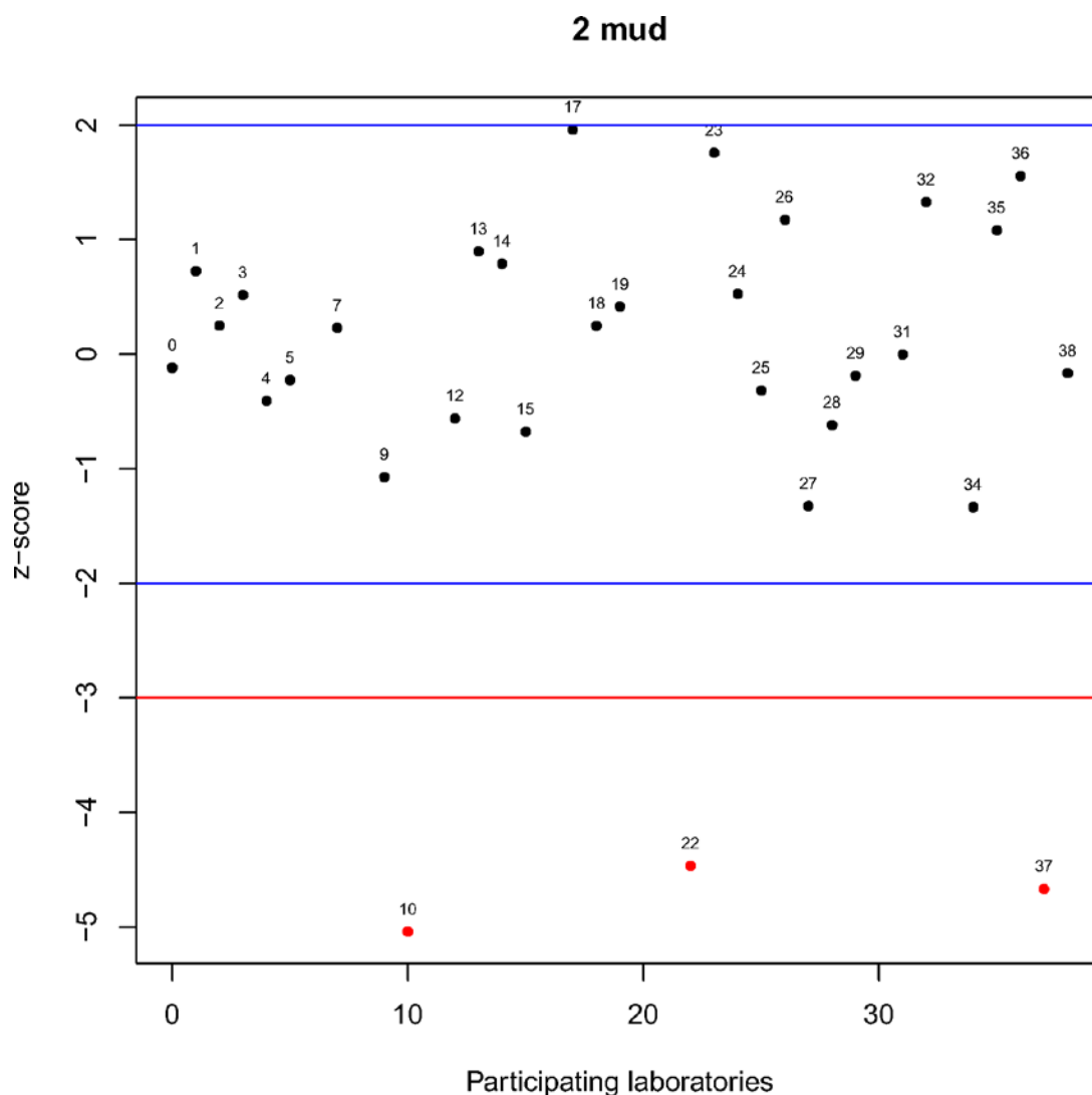
Figure 3.13 Results of Exercise 1 (z-score). Blue lines are equal to \pm 2 * z\text{-score} and red lines are equal to \pm 3 * z\text{-score} . Black dots represent results classified 'S', blue dots those classified 'Q' and red dots the results classified 'U'.
