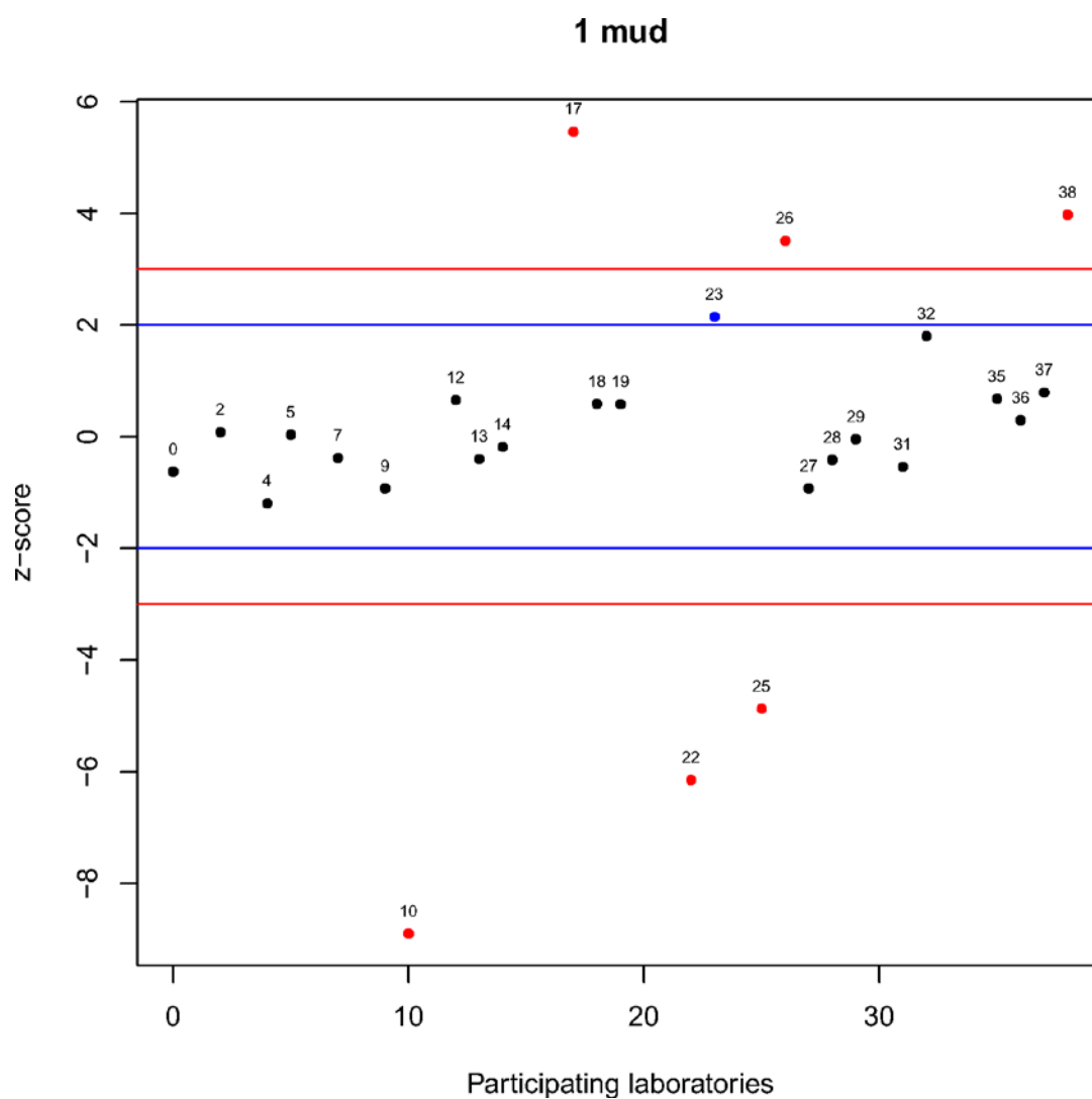
Figure 3.5 Results of Exercise 1 (z-score). Blue lines are equal to \pm 2 \cdot z\text{-score} and red lines are equal to \pm 3 \cdot z\text{-score} . Black dots represent results classified 'S', blue dots those classified 'Q' and red dots the results classified 'U'.
