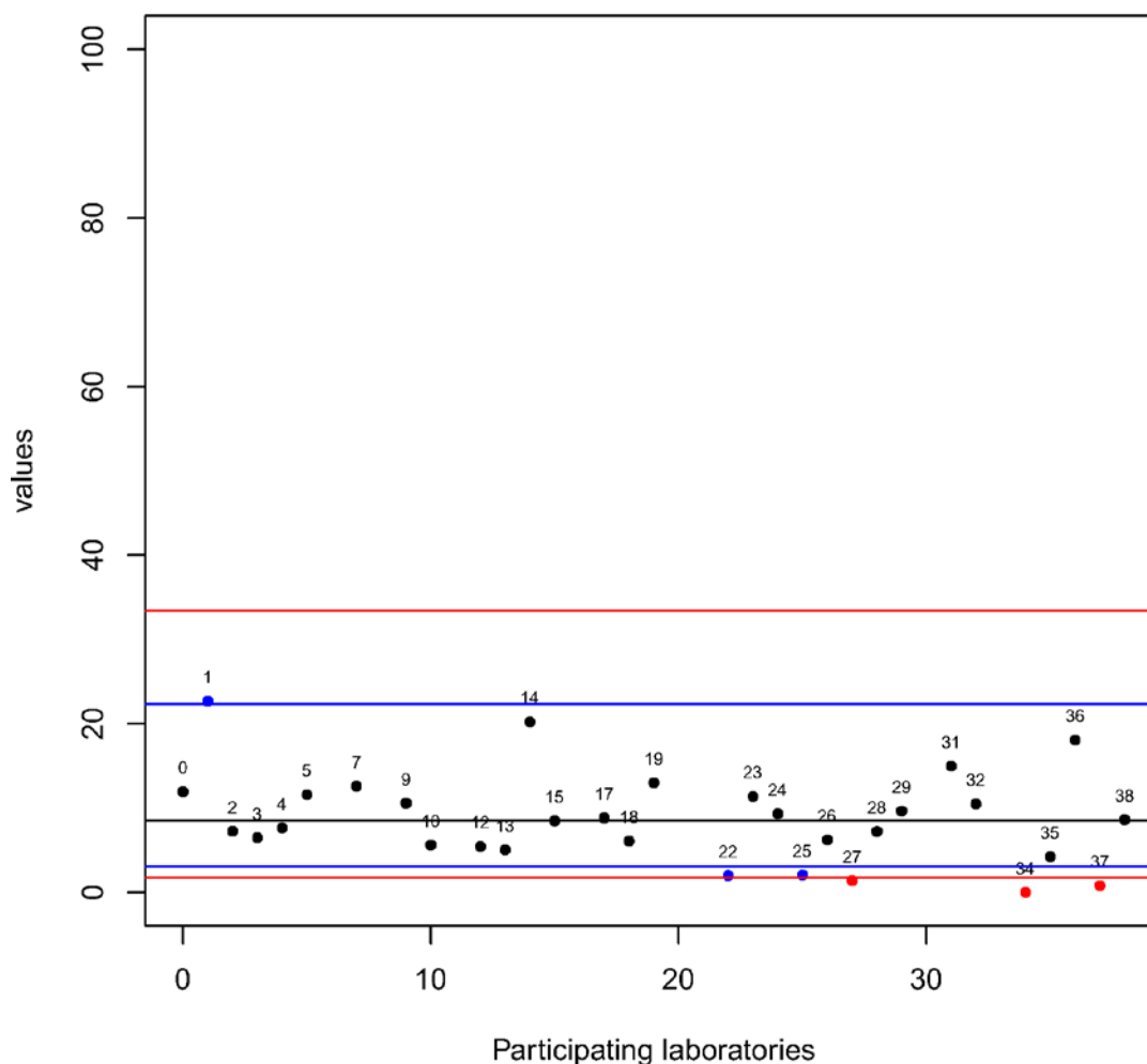
Figure 3.26 Results of Exercise 1 (%). Black line is equal to median x_i , blue lines are equal to \pm 2 * z-score and red lines are equal to \pm 3 * z-score. Black dots represent results classified 'S', blue dots those classified 'Q' and red dots the results classified 'U'.
