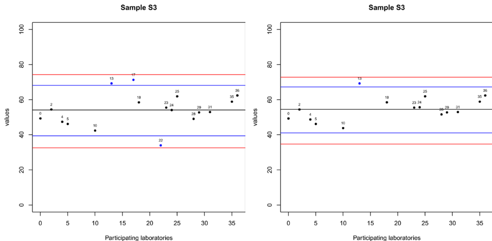
Figure 3.38 Fraction <63 μm without and with ultrasonic treatment (%). Black line is equal to median , blue lines are equal to ± 2 * z-score and red lines are equal to ± 3 * z-score . Numbers represent assigned lab number, black dots represent results classified 'S', blue dots those classified 'Q' and red dots the results classified 'U'.
